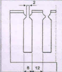
Standard Slot
